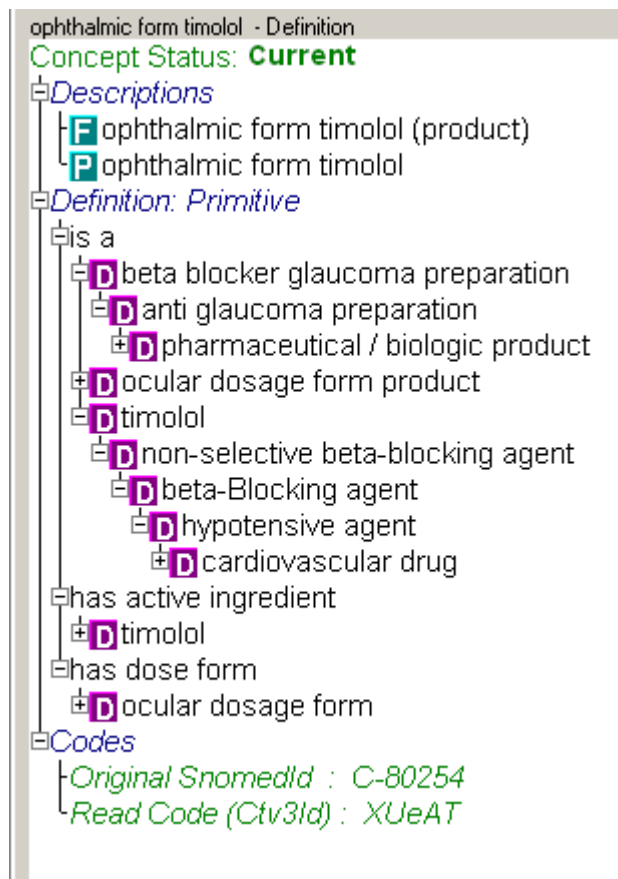
Figure 57: Timolol Supertypes
