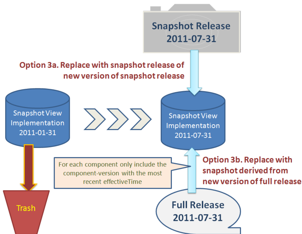
Figure 93: Updating a snapshot view by replacement
