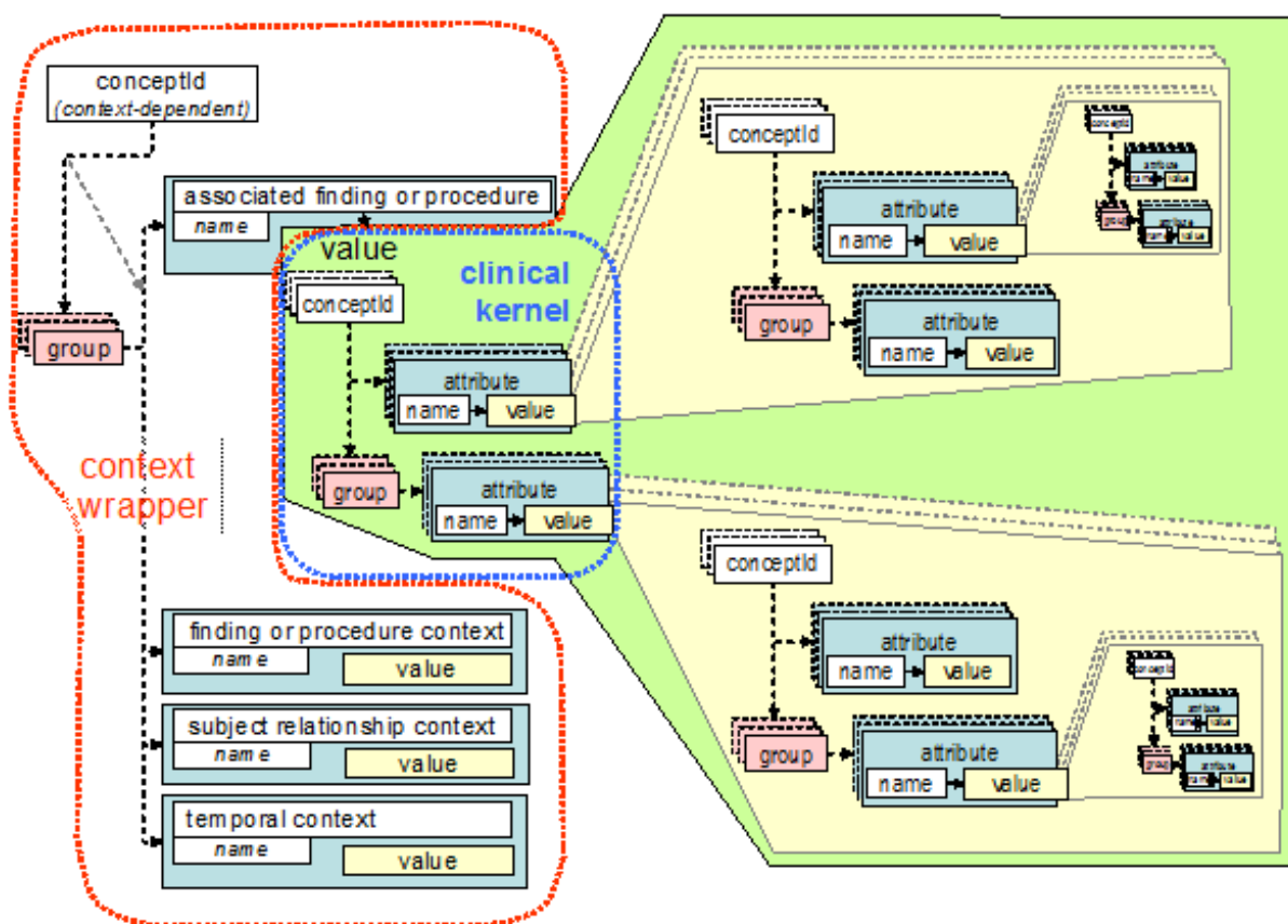
Figure 126: Illustration of the names used to refer to parts of an expression that represent context
