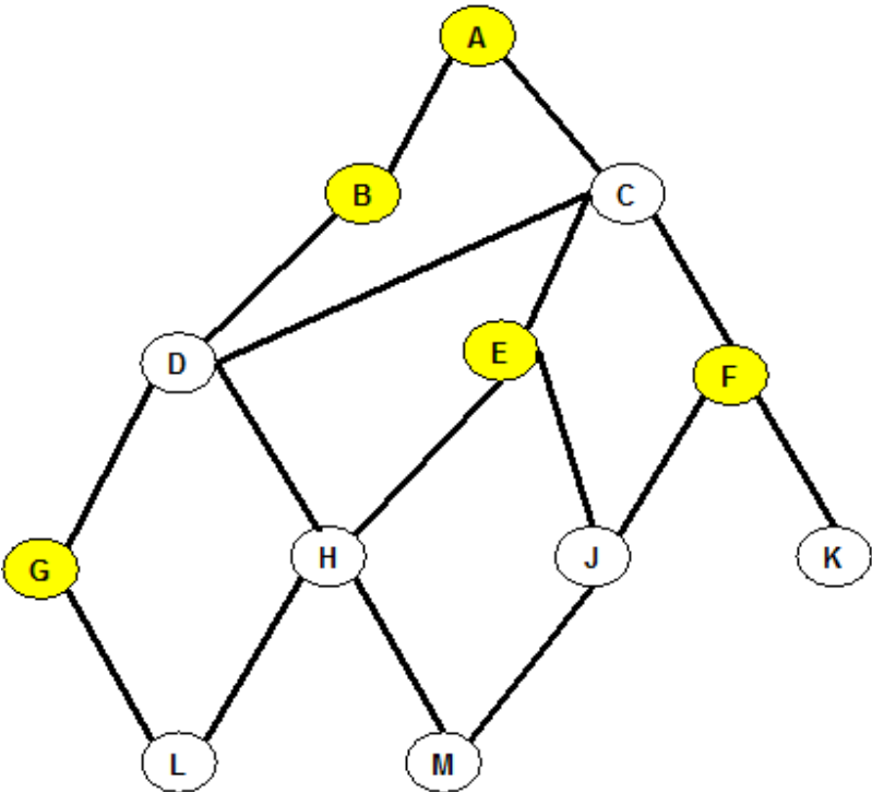
Figure 14: Example hierarchy with list of proximal supertypes
