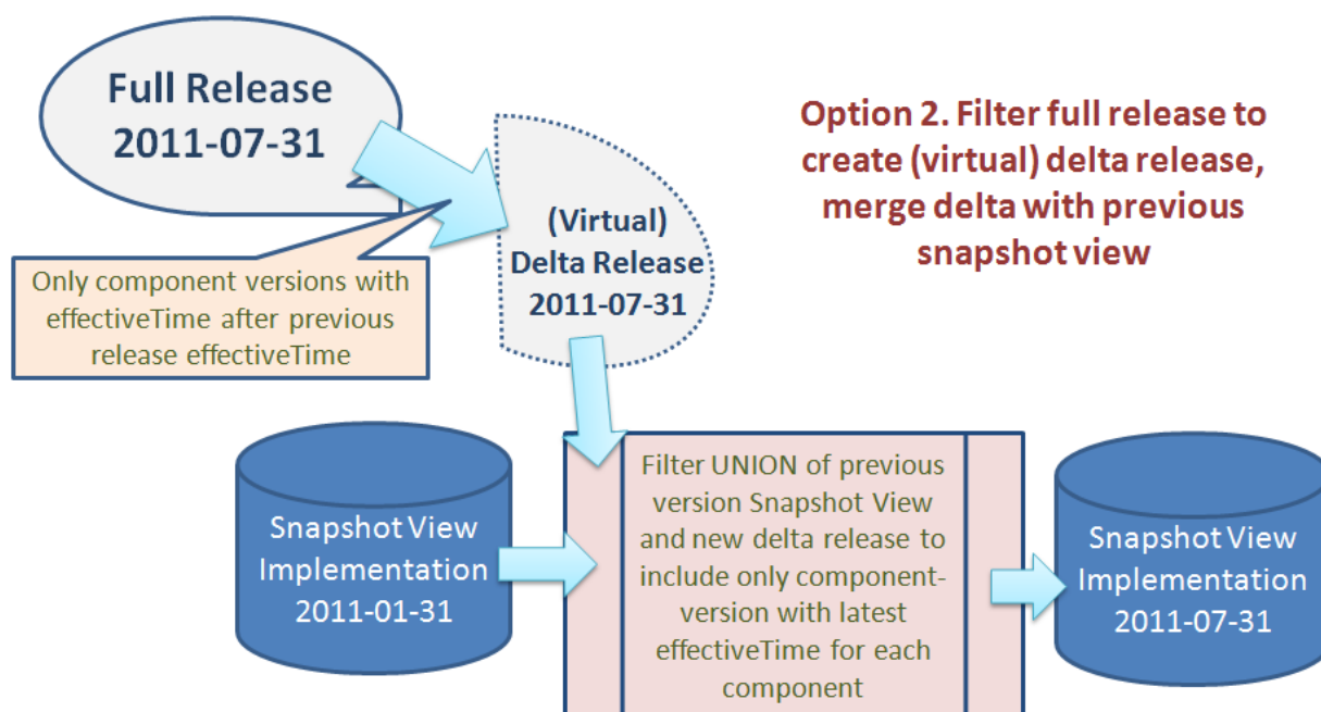
Figure 92: Updating a snapshot view using a full release
