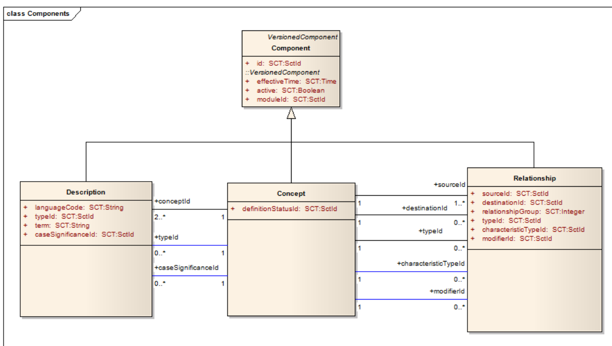
Figure 12: General Abstract Logical Model of a SNOMED CT concept definition
